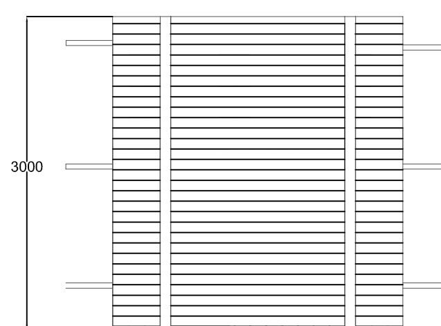
Timber Acoustic Fence 3m High Close Boarded Along the Southern Elevation
